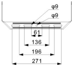
Mounting Holes
